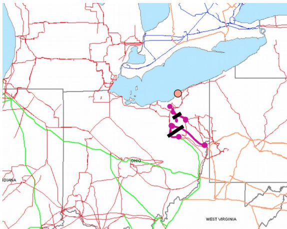
Figure 10: Cleveland and Akron supply cuts, through Sammis-Star Trip (NAERC 2004, under fair use)
