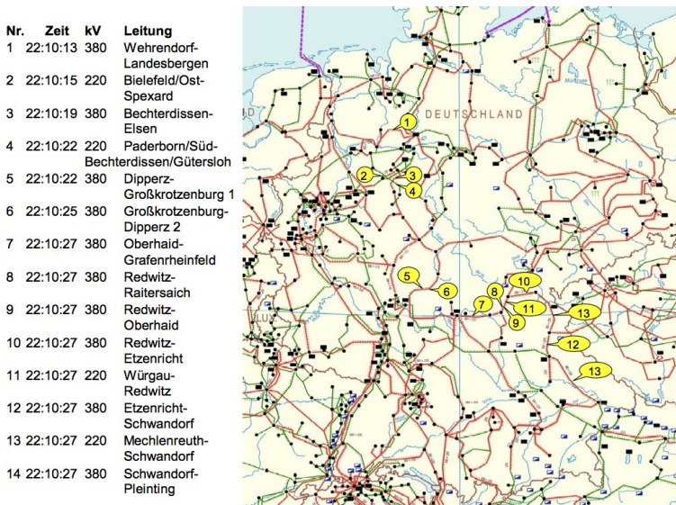
Figure 20: The first 14 lines tripped within 14 seconds (EON 2006)
