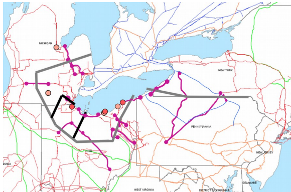
Figure 16: Cleveland and Toledo islanded at 4:41-4:49 minutes (NAERC 2004, under fair use)
