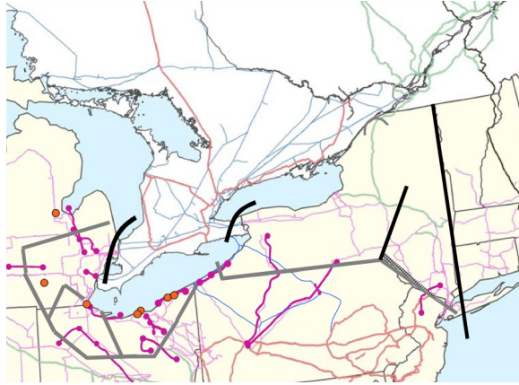
Figure 19: New York and New England separate: multiple islands form (NAERC2004, under fair use)
