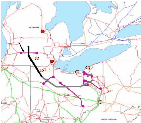
Figure 14: Eastern Michigan trips at 4:39-4:40 minutes (NAERC 2004, under fair use)
