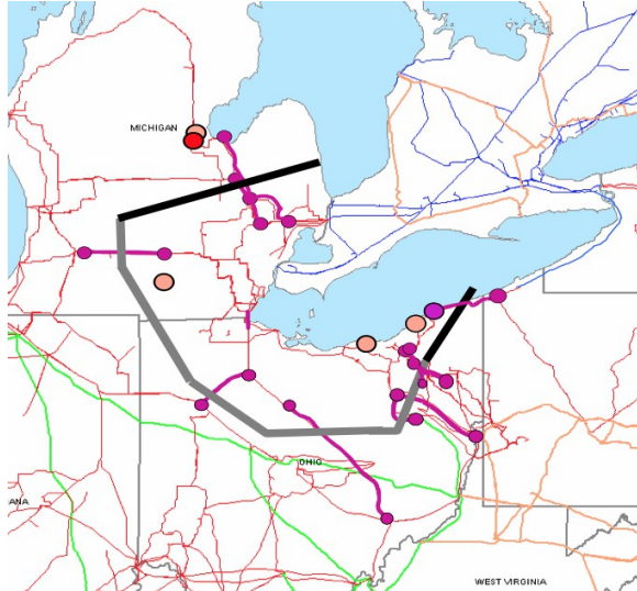
Figure 15: Michigan Trips and Ohio separates from Pennsylvania at 4:39-4:41.6 minutes (NAERC 2004, under fair use)
