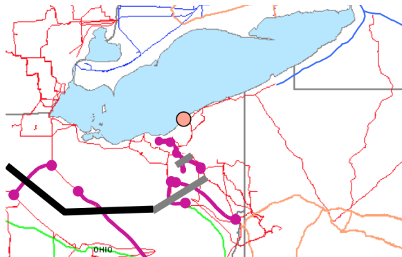
Figure 12: Ohio 345kV line trips at 3:02-3:10 minutes (NAERC 2004, under fair use)
