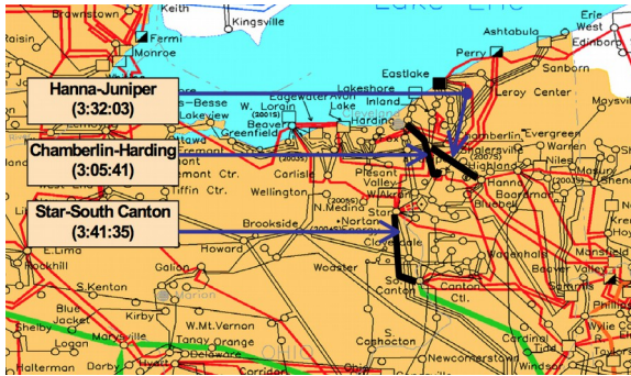
Figure 9: Three 345kV line trips (NERC 2004, under fair use)
